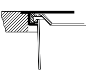
Flush mounted
